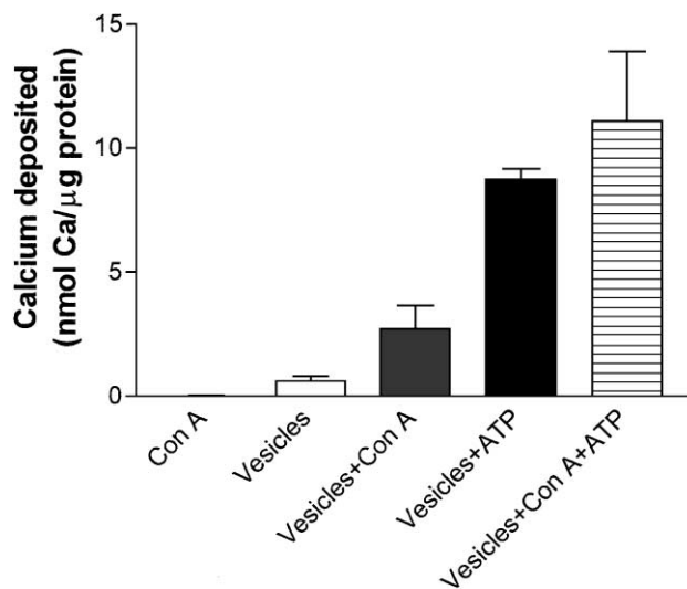
Fig. 4. Effects of ATP and Con A on calcification. Ca deposition was measured as the amount of ^{45}\text{Ca} deposits trapped on Millipore filters. ^{45}\text{CaCl}_2 deposition on the filter in the absence of vesicles was used as a blank to subtract from all the experimental data. Values are given as means \pm S.D. from three separate experiments. The vesicle preparation represents a pool of vesicles obtained separately from four rabbits. Details of the calcification assay are described under Experimental procedures. Ca deposition is expressed as nmol Ca/ \mu\text{g} protein at the end of 5-h incubation period.
